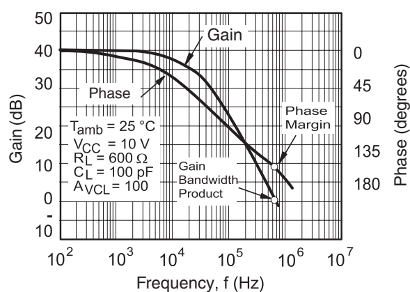
Figure 11. Gain and phase vs. frequency ( R_L = 600\ \Omega )
