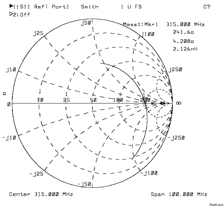
Figure 4-9 Sparam_measured_200M
