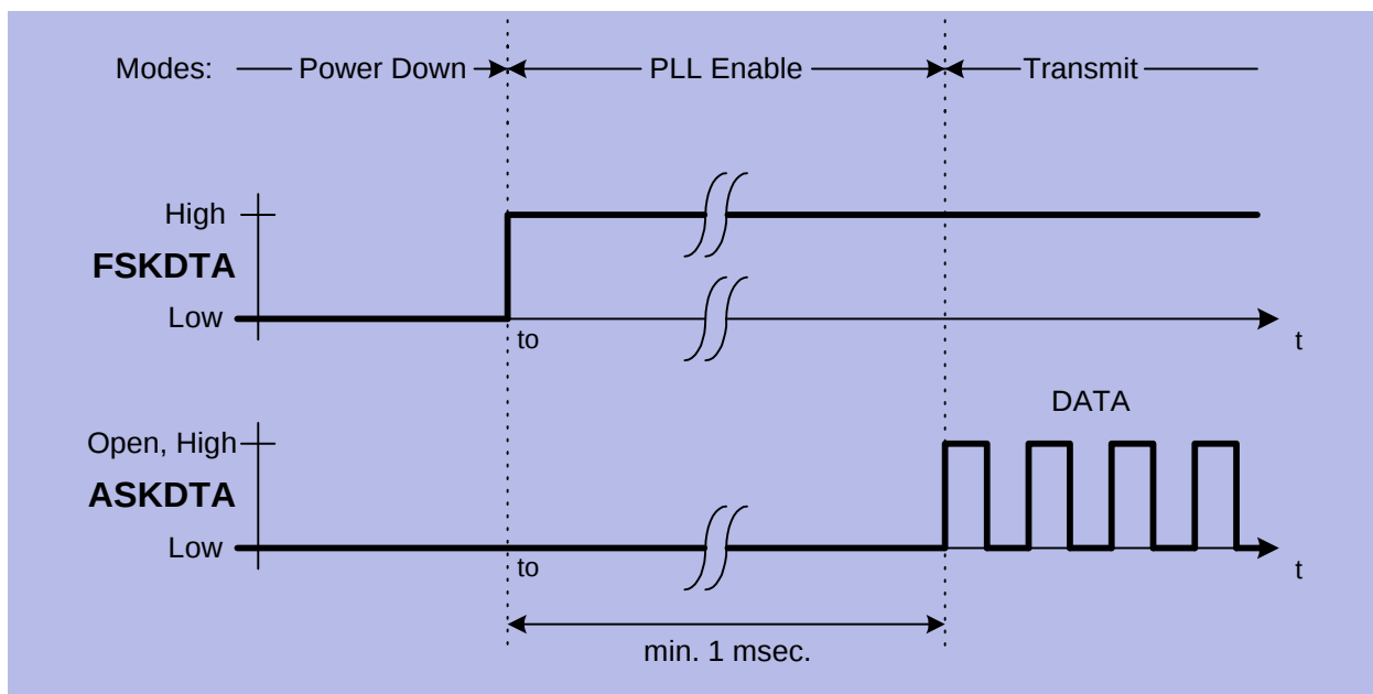
Figure 3-6 ASK Modulation
