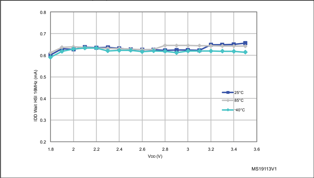
Figure 16. Typical I_{DD(Wait)} from RAM vs. V_{DD} (HSI clock source), f_{CPU} = 16\text{ MHz}
