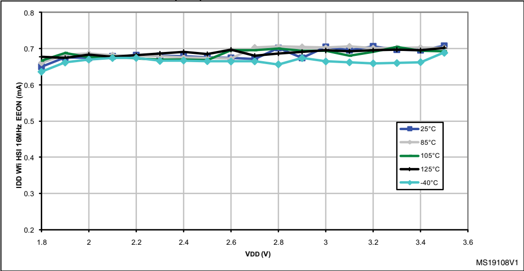
Figure 17. Typical I_{DD(Wait)} from Flash (HSI clock source), f_{CPU} = 16\text{ MHz}
