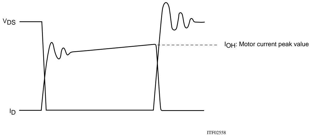
Figure 2 Output Current, I_D , and Voltage, V_{DS} , Waveforms 2 of the STK672-400 when Driving a 2-Phase Stepping Motor with Constant Current Chopping
