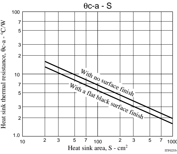
Figure 3 Heat sink area (thickness: 2mm) - \theta_{c-a}
