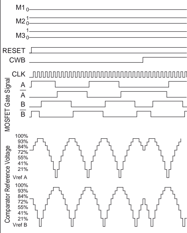
2W1-2 Phase Excitation Timing Chart (M3=0)
