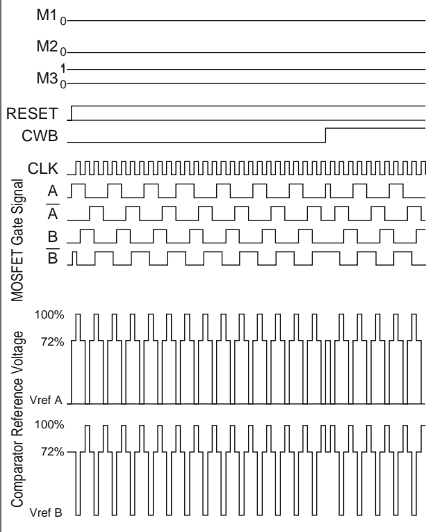
1-2 Phase Excitation Timing Chart (M3=0)
