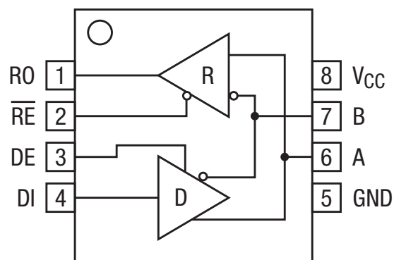
SP3485 Pinout (Top View)
