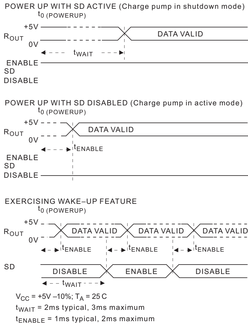
Figure 11: Wake-Up Timing
