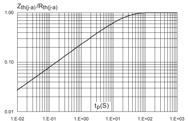
Figure 9. Relative variation of thermal impedance junction to ambient versus pulse duration (printed circuit board FR4, S_{\text{Cu}} = 1 \text{ cm}^2 )
