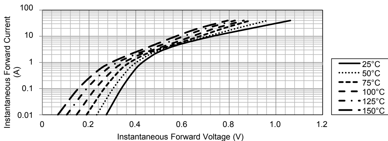
Figure 5. Typical Instantaneous Forward Characteristics (SK55B thru SK56B)
