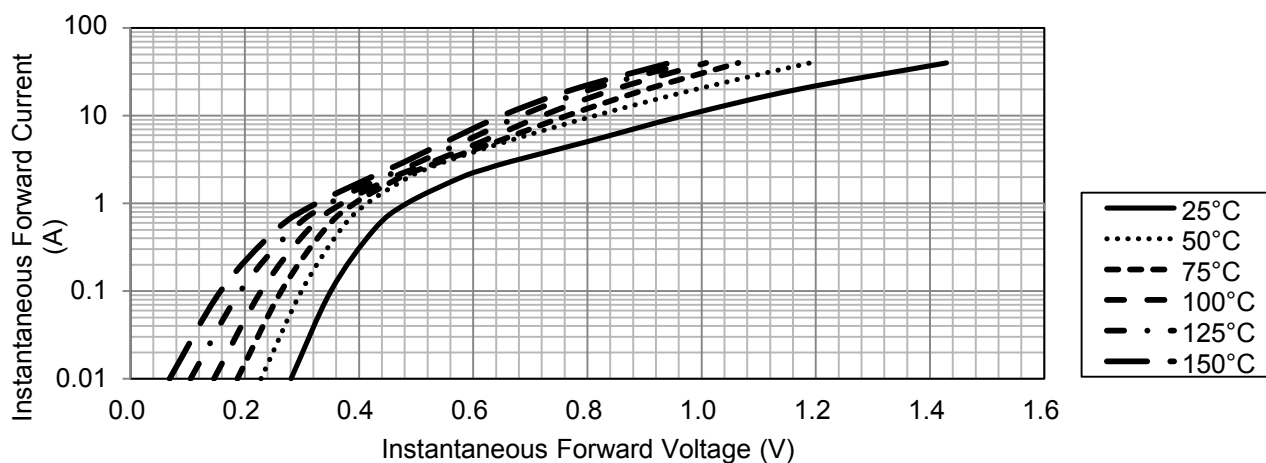
Figure 5. Typical Instantaneous Forward Characteristics (SK35 thru SK36)
