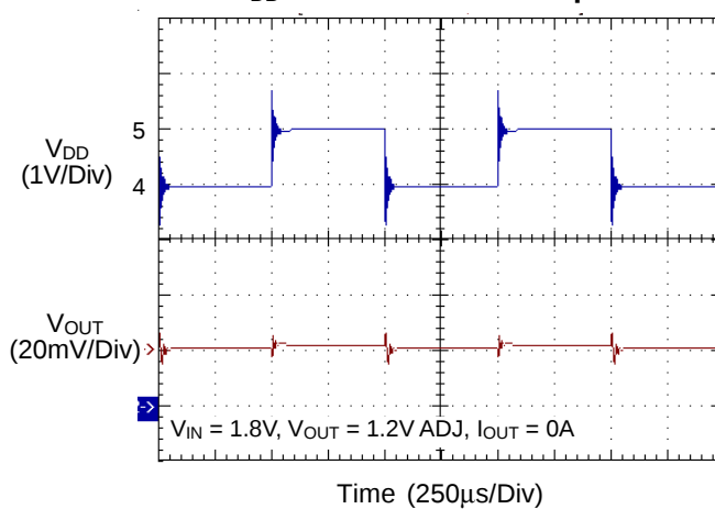
V DD Line Transient Response
