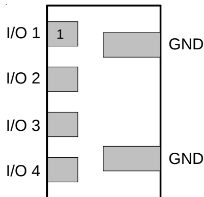
Figure 1 - Pin Configuration
