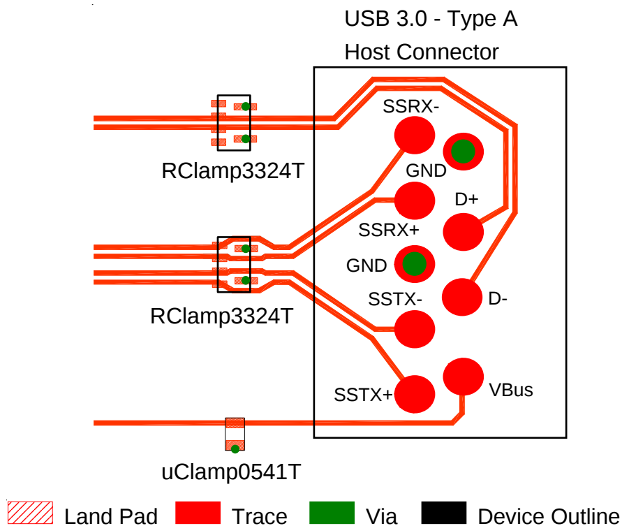
Figure 3 - USB 3.0 Layout (Type A Host Connector)
