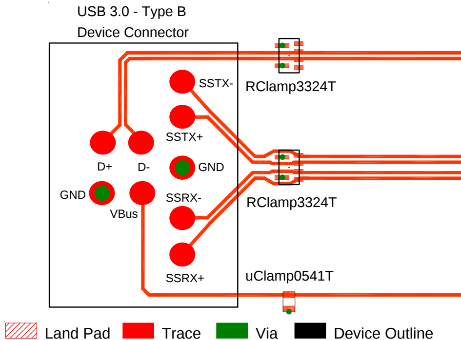
Figure 4 - USB 3.0 Layout (Type B Device Connector)
