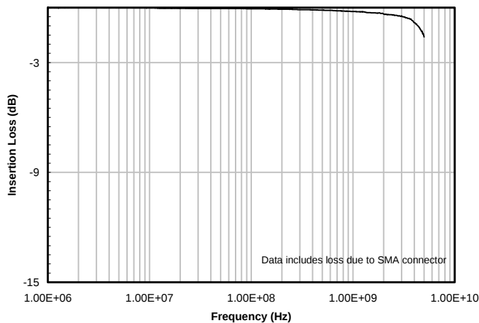
Typical Insertion Loss S21 (5GHzZ)
