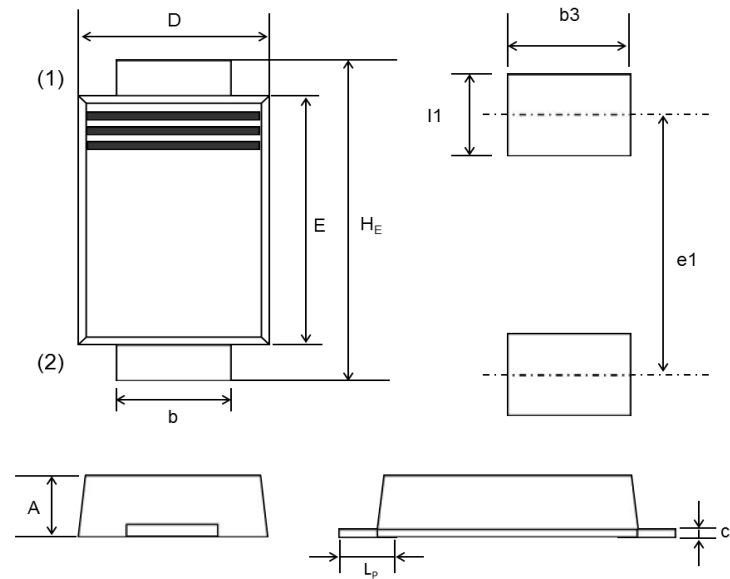
SOD-128, (PMD™)
