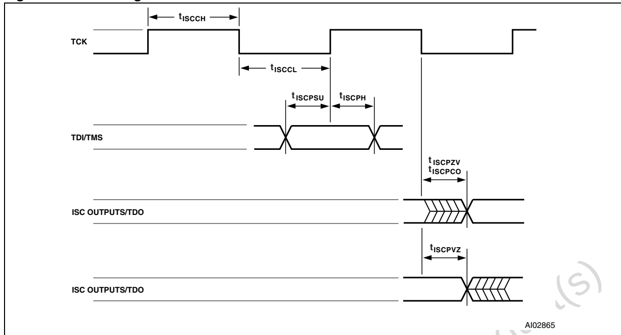
Figure 50. ISC Timing
