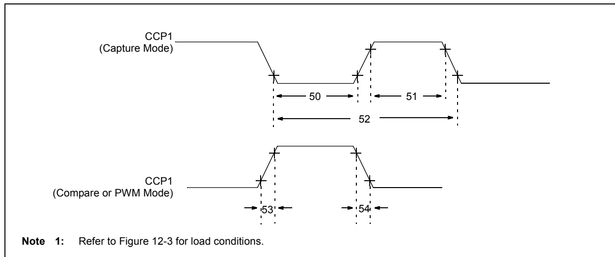
FIGURE 12-9: CAPTURE/COMPARE/PWM TIMINGS (1)
