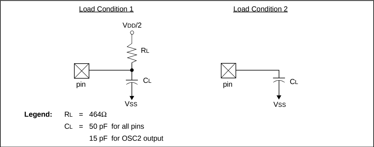
FIGURE 15-3: LOAD CONDITIONS
