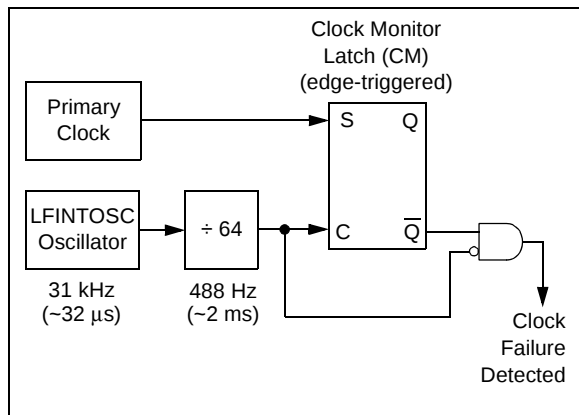
FIGURE 3-8: FSCM BLOCK DIAGRAM
