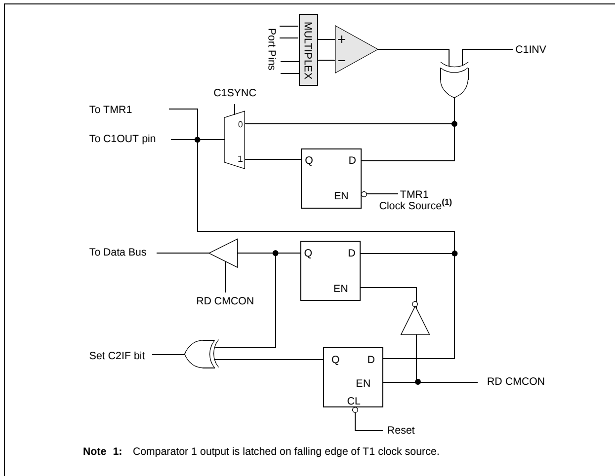
FIGURE 7-5: PIC12F635 COMPARATOR C1 OUTPUT BLOCK DIAGRAM
