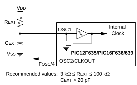
FIGURE 3-5: RC MODE
