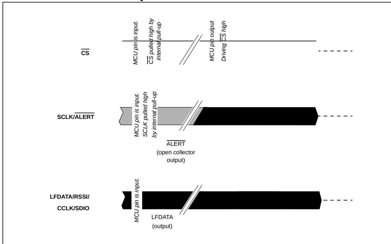
FIGURE 11-16: POWER-UP SEQUENCE
