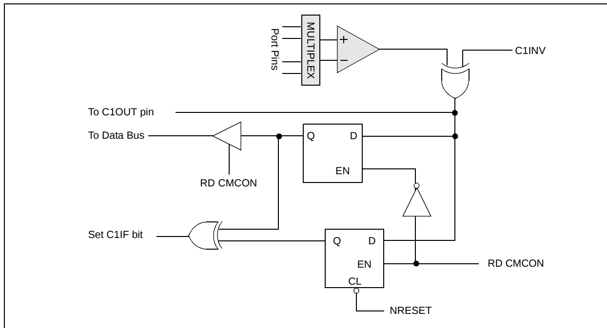
FIGURE 7-6: PIC16F636/639 COMPARATOR C1 OUTPUT BLOCK DIAGRAM
