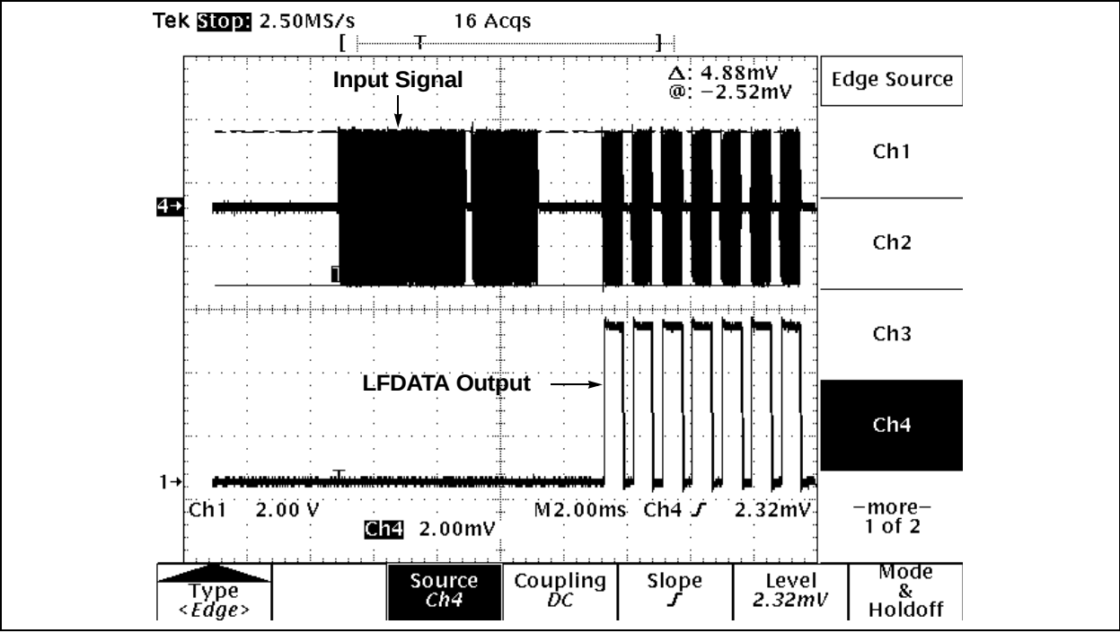
FIGURE 11-11: INPUT SIGNAL AND DEMODULATOR OUTPUT (WHEN OUTPUT ENABLE FILTER IS ENABLED AND INPUT MEETS FILTER TIMING REQUIREMENTS)
