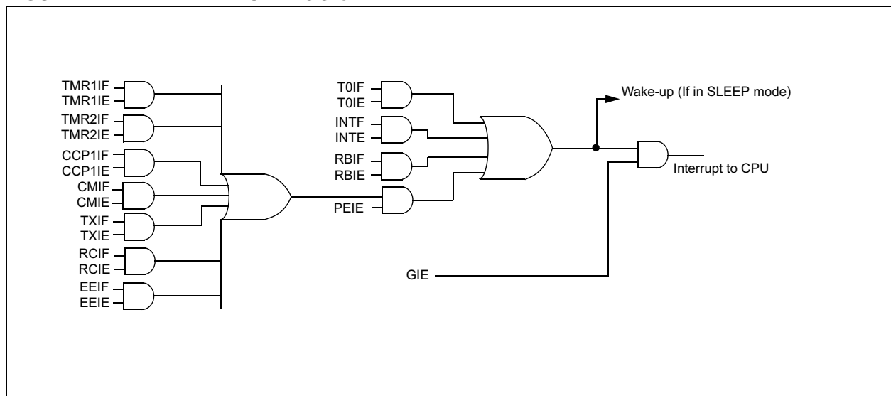
FIGURE 14-14: INTERRUPT LOGIC
