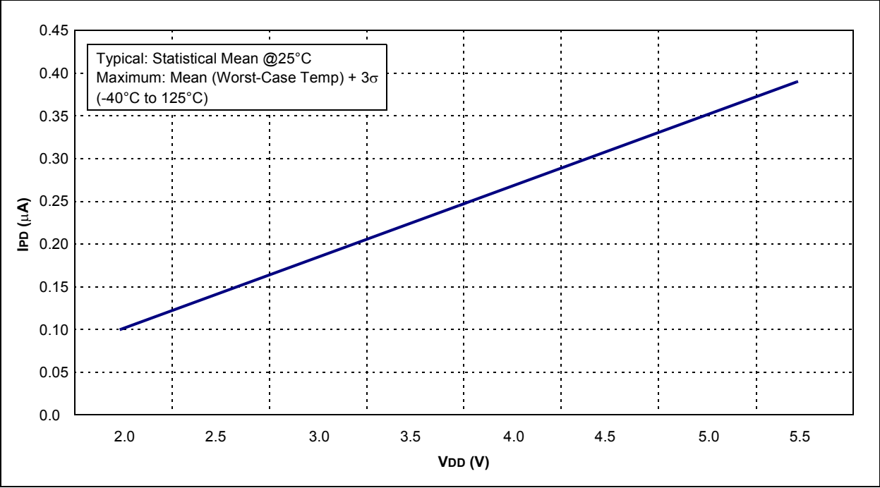
FIGURE 15-6: MAXIMUM I_{PD} vs. V_{DD} (SLEEP MODE, ALL PERIPHERALS DISABLED)
