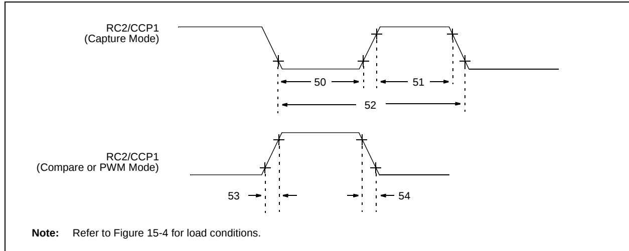
FIGURE 15-9: CAPTURE/COMPARE/PWM TIMINGS
