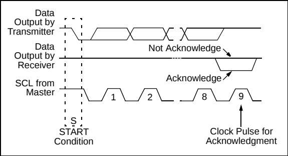
FIGURE 9-9: SLAVE-RECEIVER ACKNOWLEDGE
