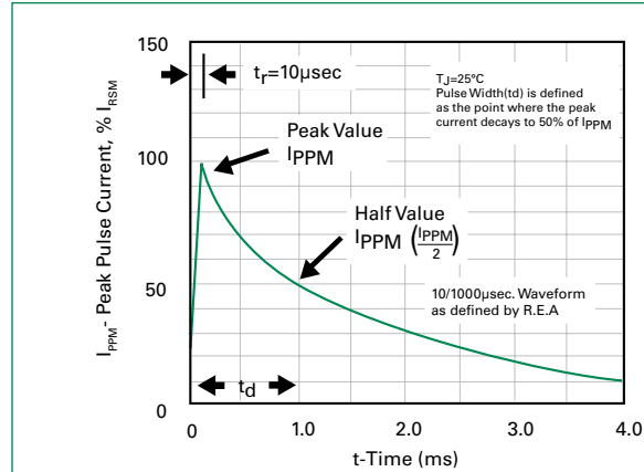
Figure 4 - Pulse Waveform
