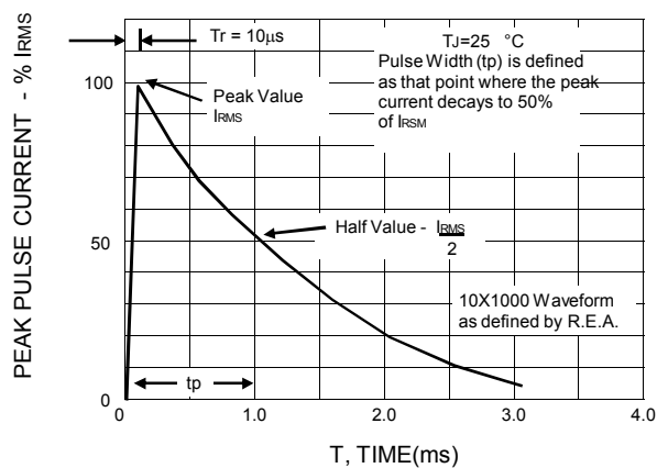
FIG.5 - PULSE WAVEFORM
