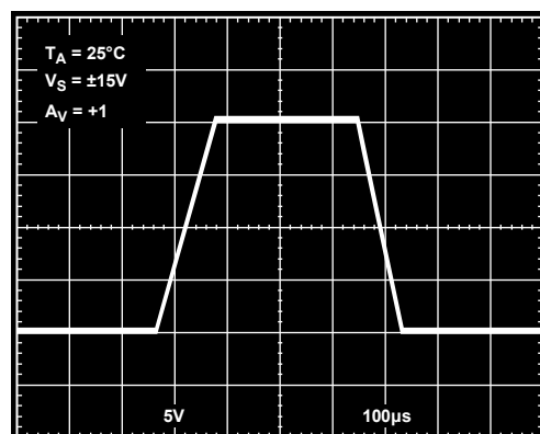
Figure 25. Large Signal Transient Response
