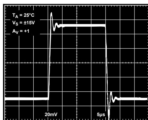
Figure 27. Small Signal Transient Response, C_{LOAD} = 1\text{ nF}
