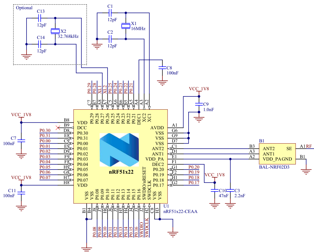
Figure 35 CEAA WLCSP with low voltage mode setup
