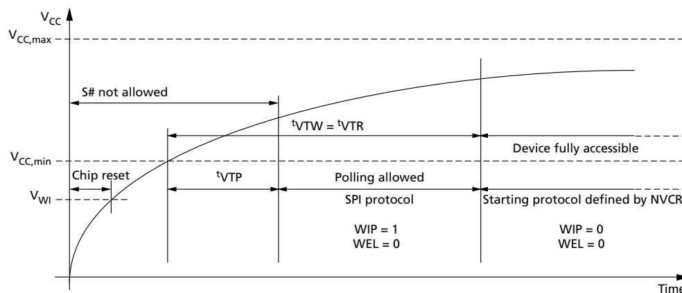
Figure 39: Power-Up Timing
