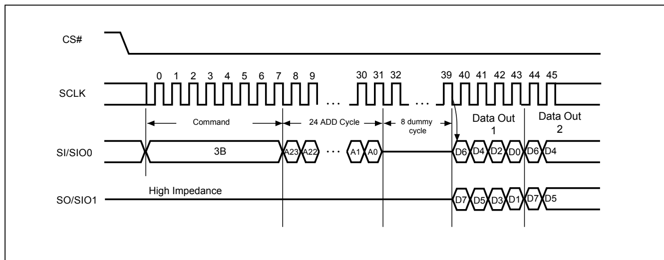
Figure 26. Dual Read Mode Sequence (Command 3B)
