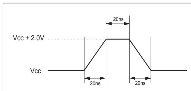
Figure 84. Maximum Positive Overshoot Waveform
