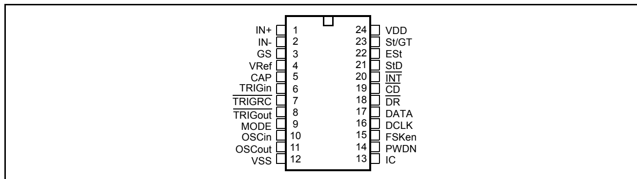
Figure 2 - Pin Connections
