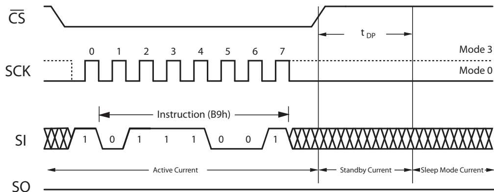
Figure 10 – Enter Sleep Mode (SLEEP) Timing
