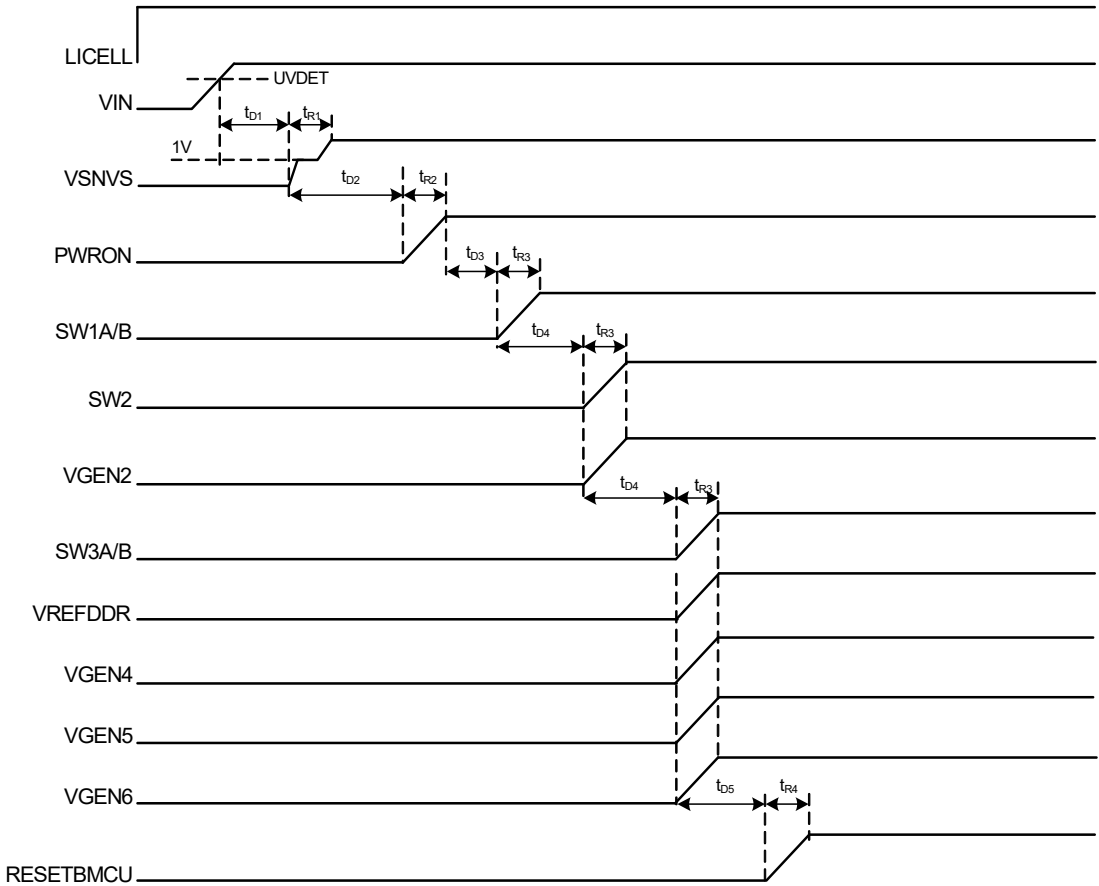
Figure 6. Default start-up sequence
