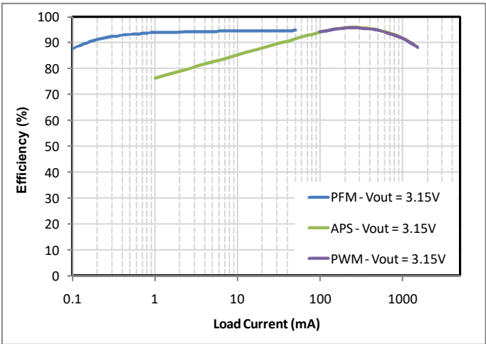
Figure 14. SW2 efficiency waveforms
