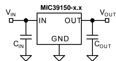
Figure 1. Capacitor Requirements
