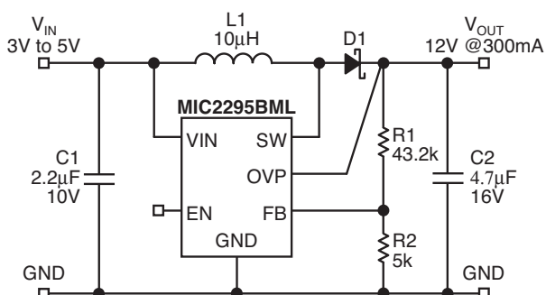
3V IN to 5V IN to 12V OUT @ 300mA
