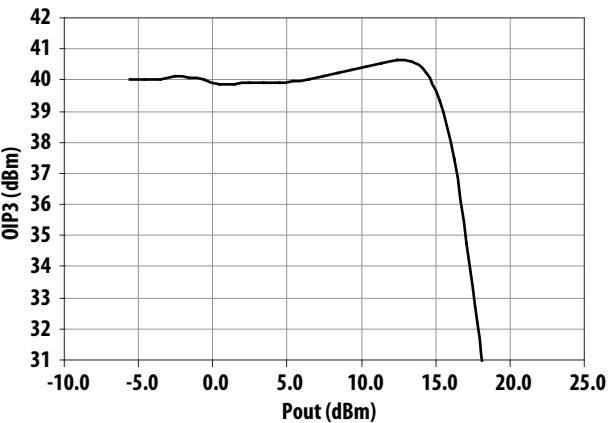
Figure 23. OIP3 vs Output Power at 1900MHz
