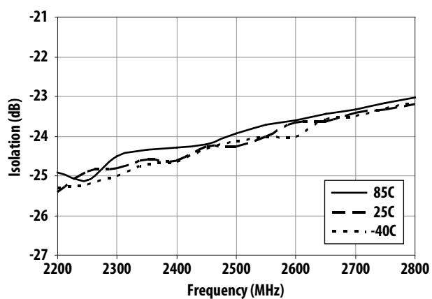
Figure 39. Isolation vs Frequency and Temperature
