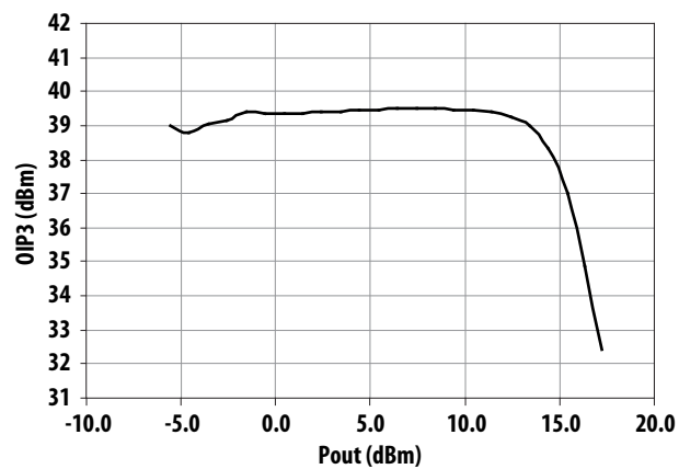
Figure 32. OIP3 vs Output Power at 1900MHz
