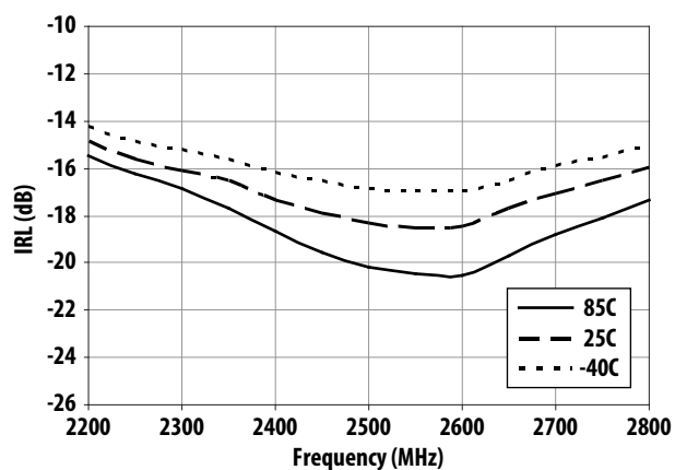
Figure 37. IRL vs Frequency and Temperature
