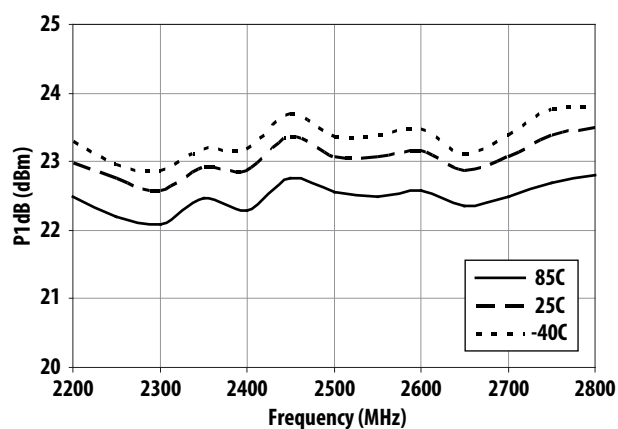
Figure 35. P1dB vs Frequency and Temperature
