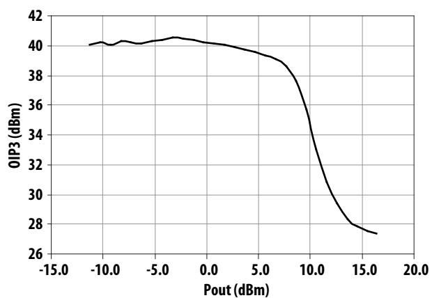
Figure 14. OIP3 vs Output Power at 450MHz
