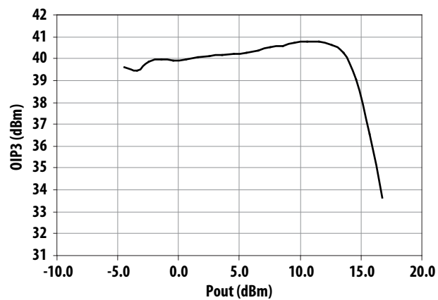
Figure 41. OIP3 vs Output Power at 1900MHz
