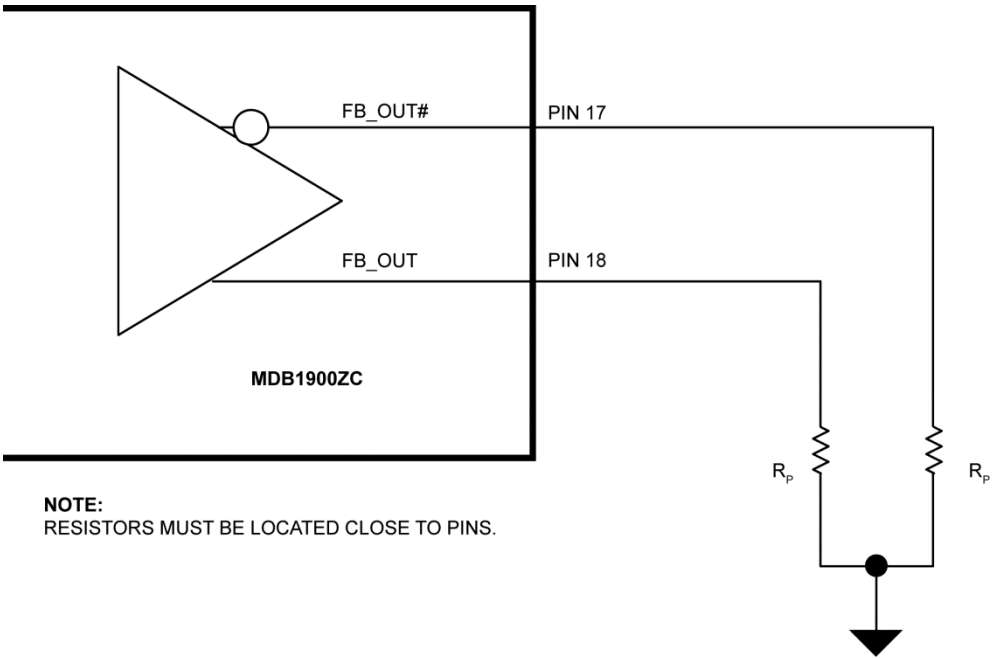
Figure 1. Feedback Termination
