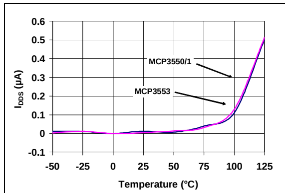
FIGURE 2-24: I_{DS} vs. Temperature.
