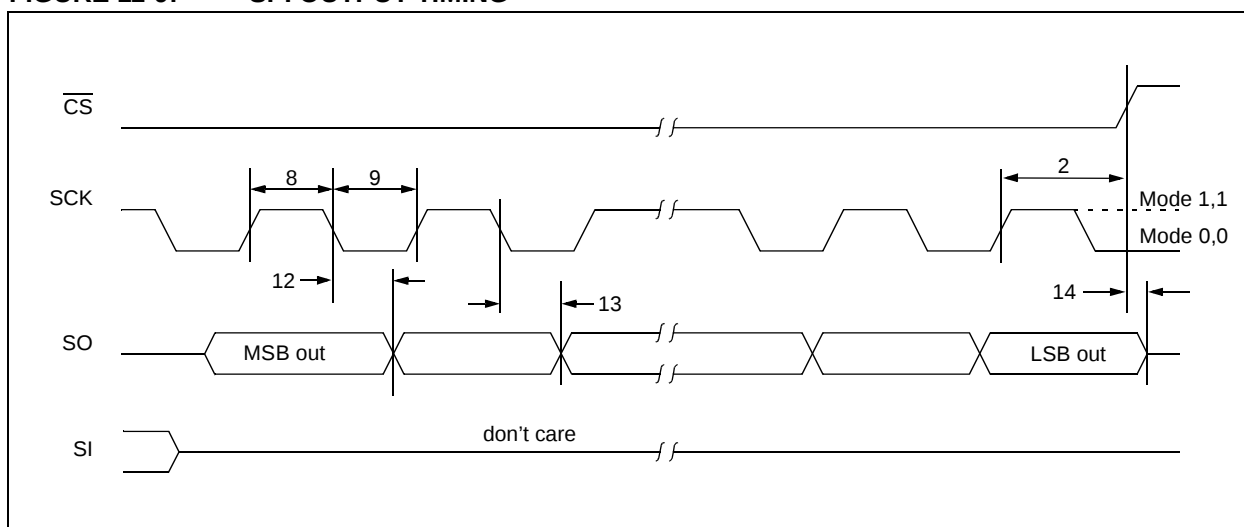
FIGURE 11-9: SPI OUTPUT TIMING
