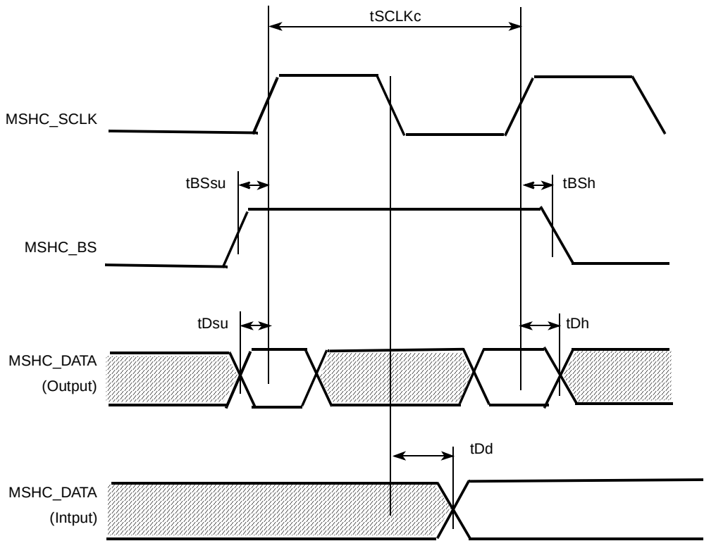
Figure 66. Transfer Operation Timing Diagram (Serial)
