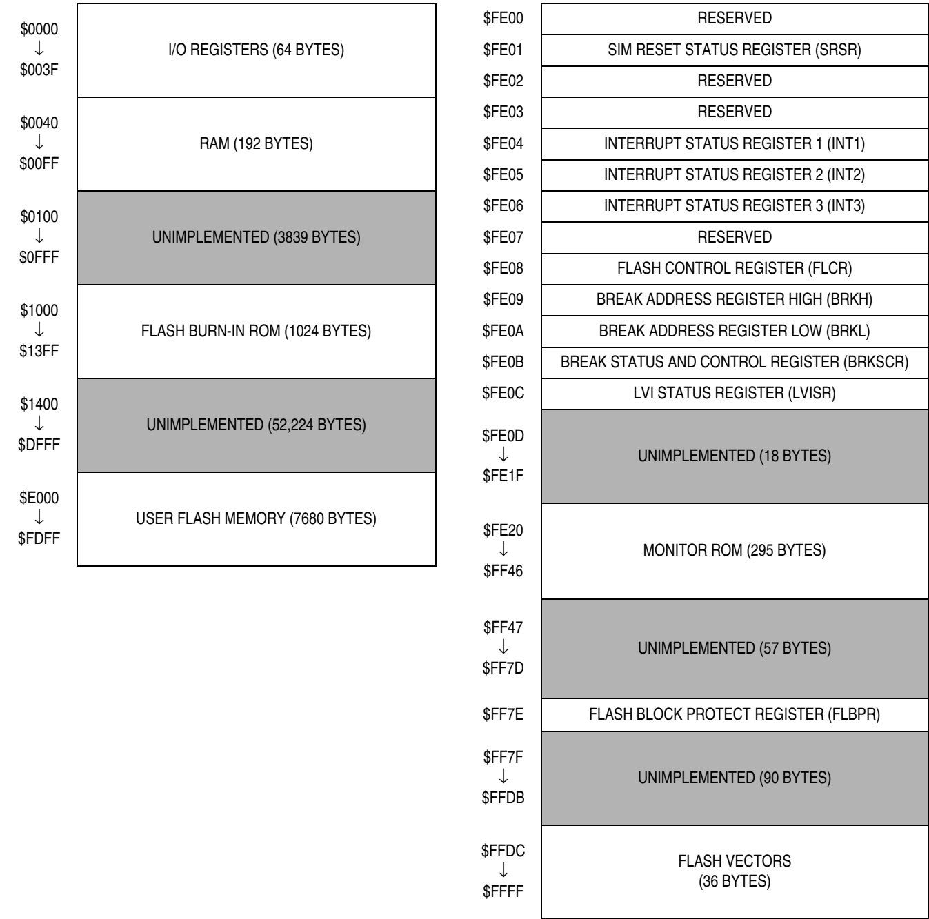
Figure 2-1. Memory Map
