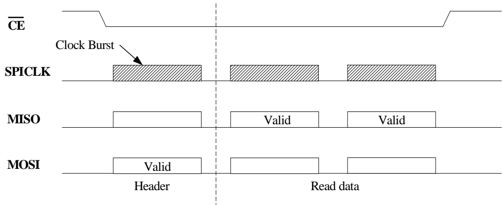
Figure 11. SPI Read Transaction Diagram
