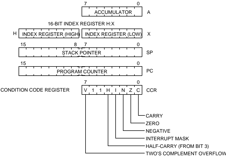
Figure 18. CPU Registers
