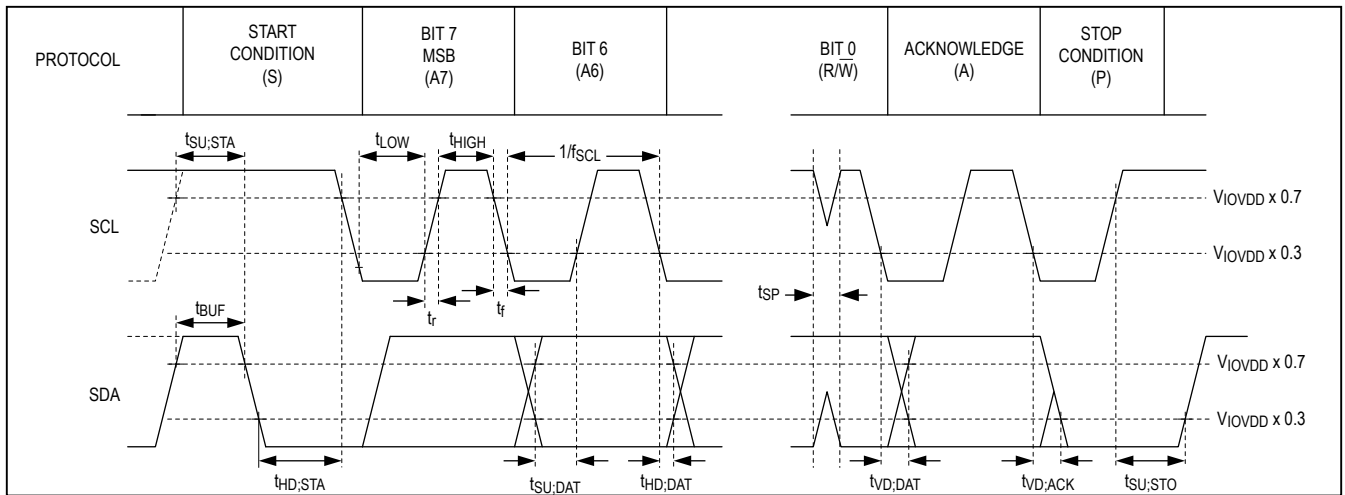
Figure 5. I²C Timing Parameters
