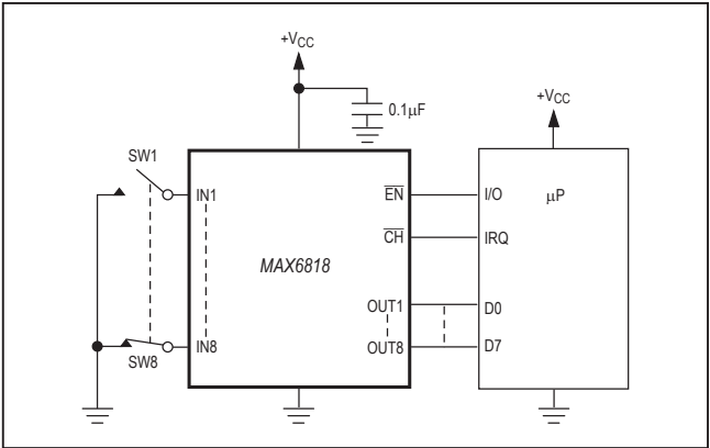
Figure 5. MAX6818 Typical μP Interfacing Circuit
