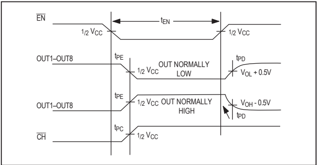
Figure 4. MAX6818 μP Interface Timing Diagram
