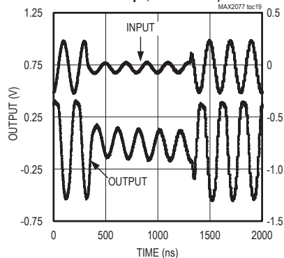
LNA OVERLOAD RECOVERY TIME ( V_{IN} = 500mV_{p-p} FOR 0.5\mu s TO 100mV_{p-p} FOR 1\mu s AND BACK TO 500mV_{p-p} FOR 0.5\mu s , GAIN = 10dB)
