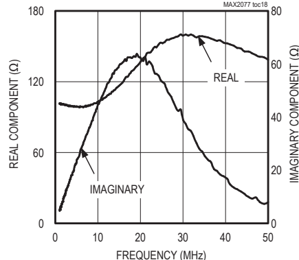
DIFFERENTIAL OUTPUT IMPEDANCE vs. FREQUENCY
