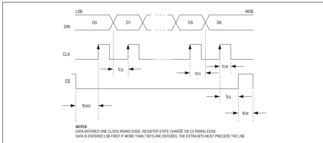
Figure 1. Shift Register Timing Diagram
