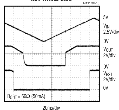
\overline{\text{RST}} WAVEFORM
