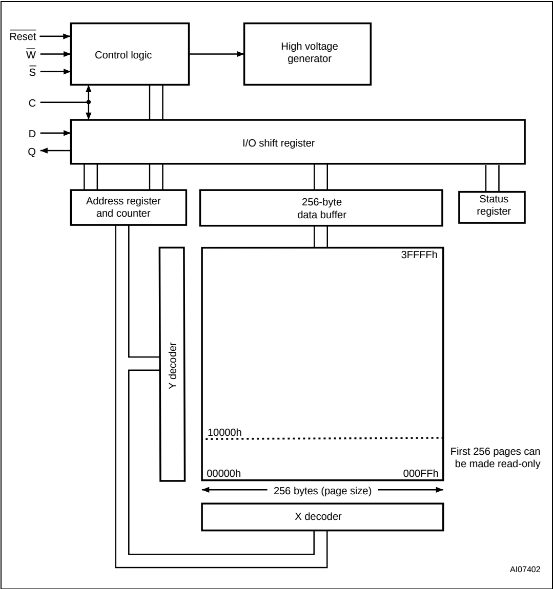
Figure 5. Block diagram
