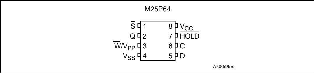
Figure 2. VDFPN connections
