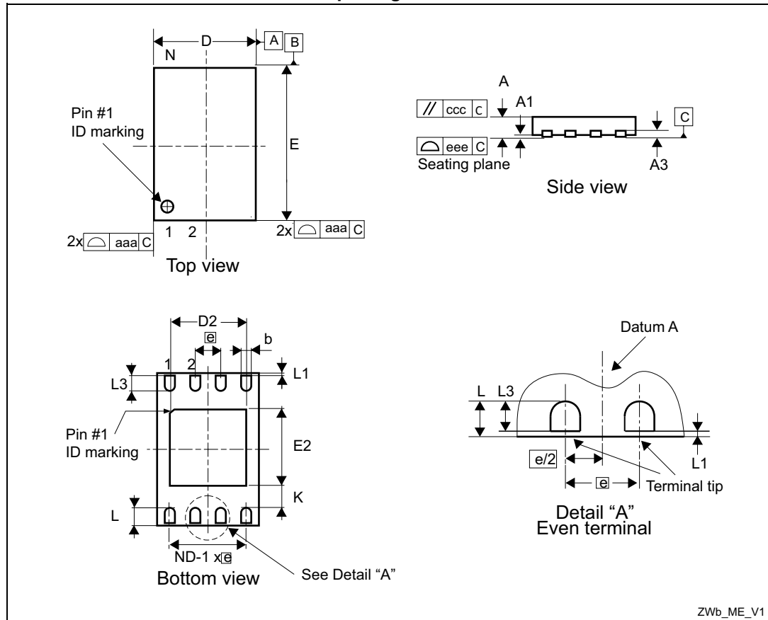
Figure 90. UDFN8 - 8-lead, 2 \times 3 mm, 0.5 mm pitch ultra thin profile fine pitch dual flat package outline
