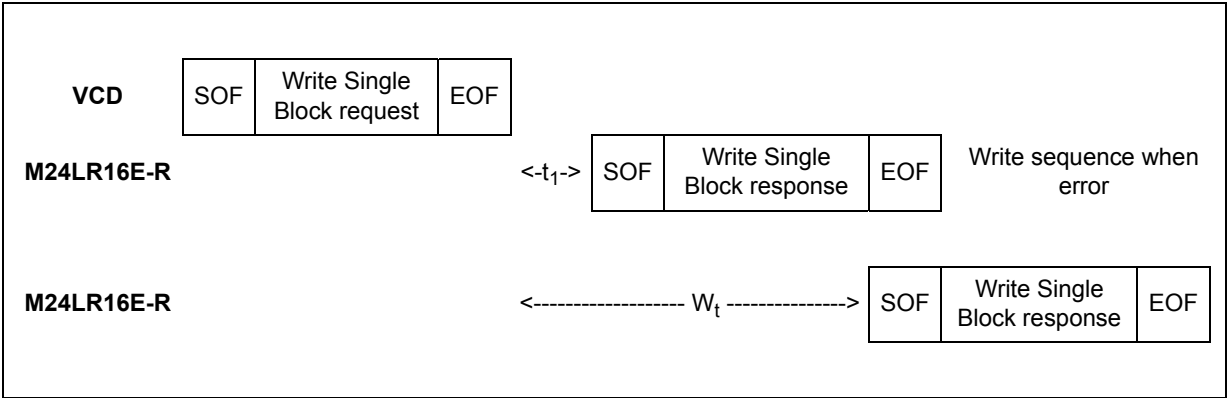
Figure 55. Write Single Block frame exchange between VCD and M24LR16E-R
