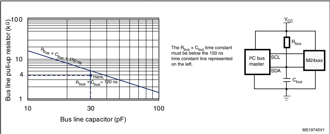
Figure 5. I 2 C Fast mode Plus ( f_C = 1\text{ MHz} ): maximum R_{bus} value versus bus parasitic capacitance ( C_{bus} )
