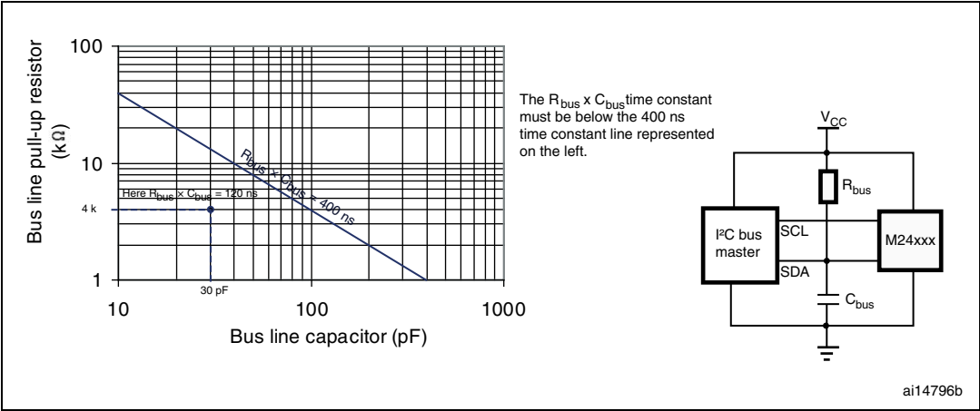
Figure 4. I 2 C Fast mode ( f_C = 400\text{ kHz} ): maximum R_{bus} value versus bus parasitic capacitance ( C_{bus} )
