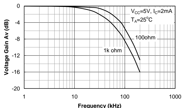
Figure 11. Frequency Response
