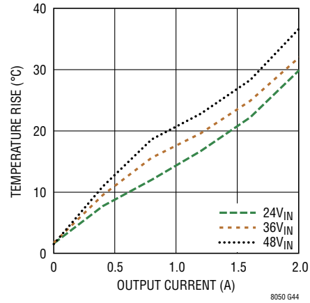
Internal Temperature Rise vs Output Current, 12V OUT
