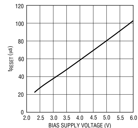
t_{\text{RESET}} vs V_{CC}
