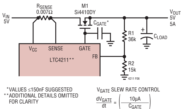
Figure 6. Using an External Capacitor at GATE for GATE Voltage Slew Rate Control
