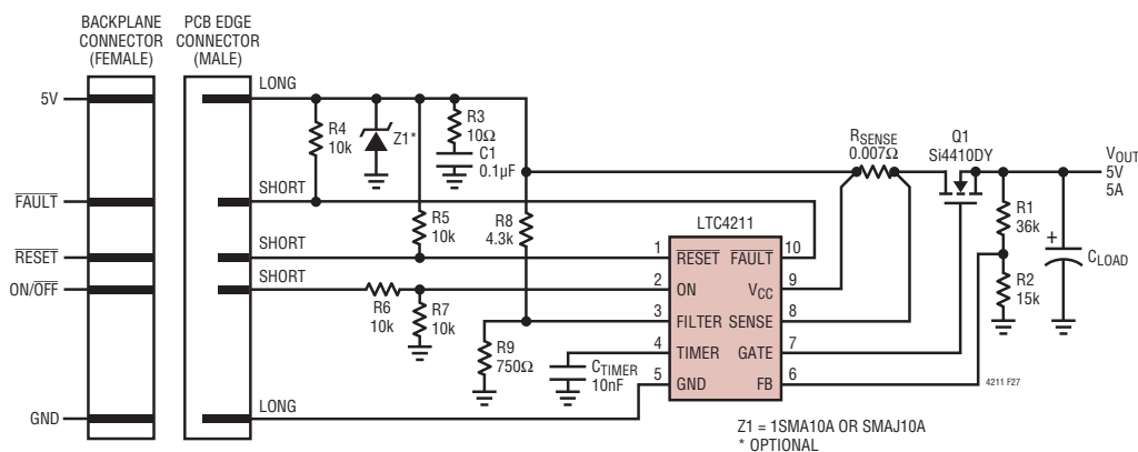
Figure 27. LTC4211MS High Side Overvoltage Protection Implementation (In Normal Mode, SLOW COMP Is Disabled. In Soft-Start Cycle, I_{SOFTSTART} Is Still 50\text{mV}/R_{SENSE} )
