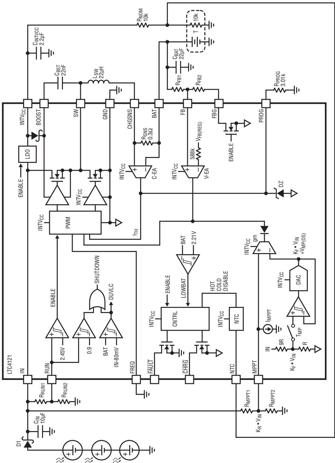
Figure 1. Block Diagram
